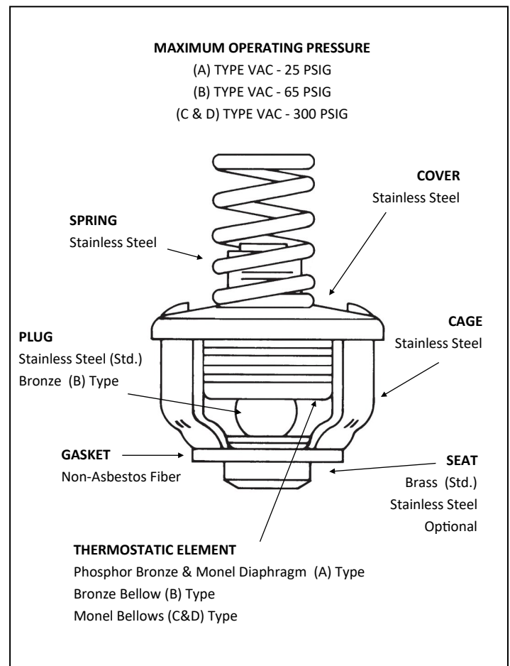
Air Vents
